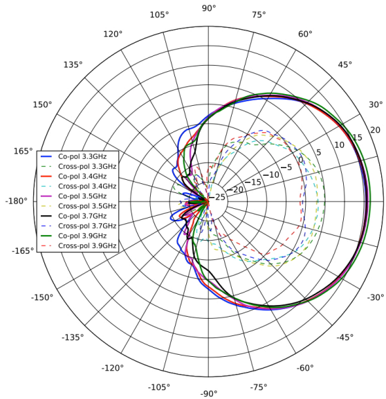
3 GHz Azimuth
