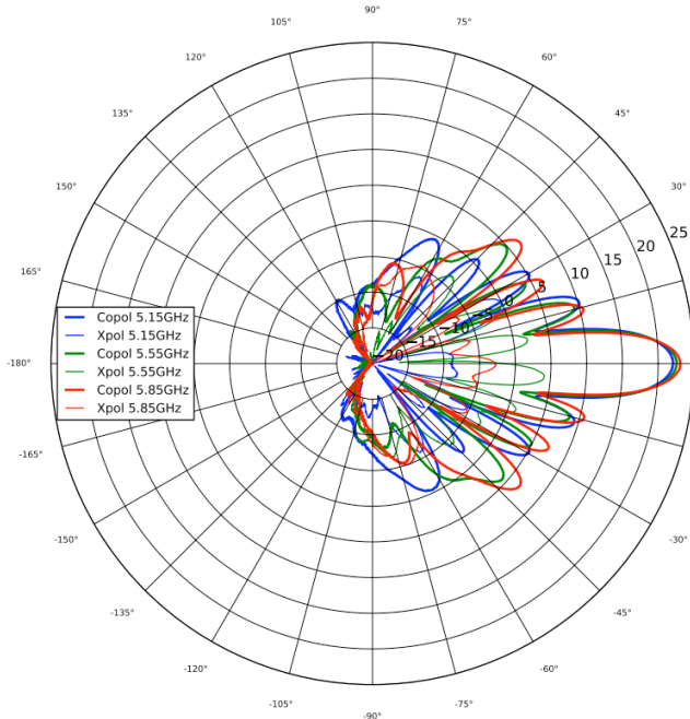
5 GHz Azimuth
