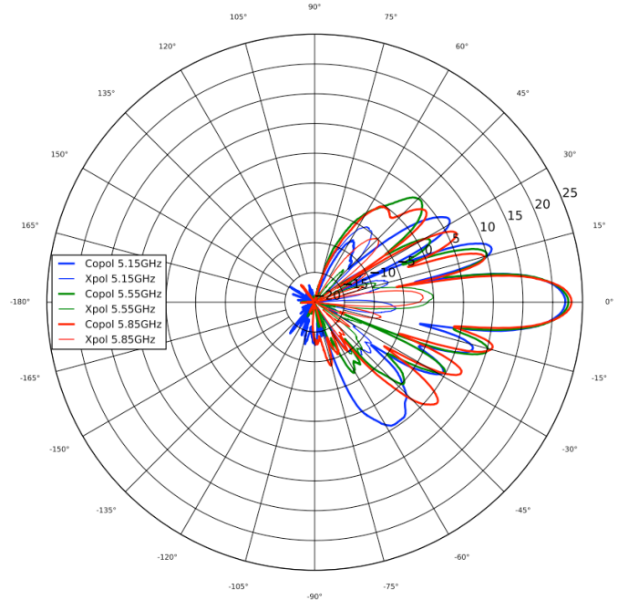
5 GHz Elevation
